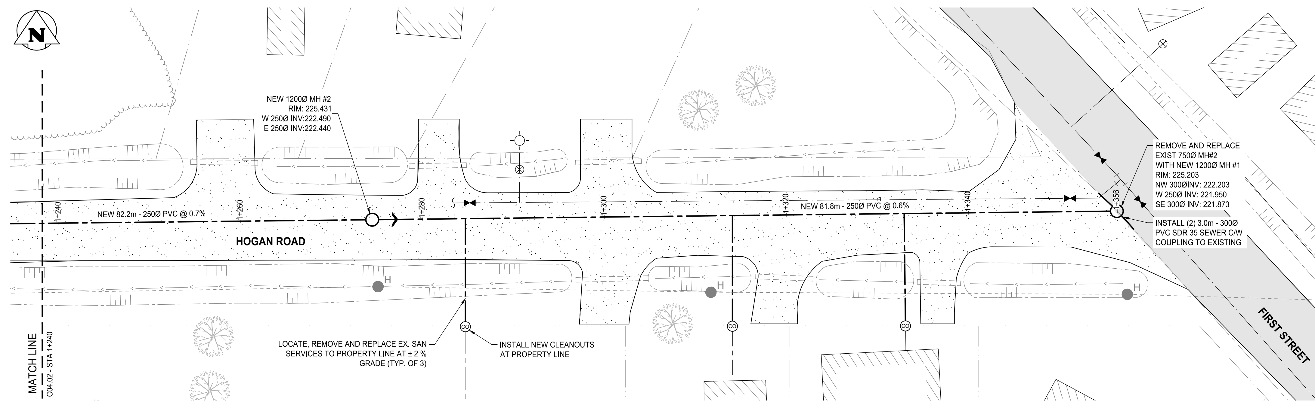
PLAN VIEW STA 1+240 TO 1+360 SCALE: 1:250
