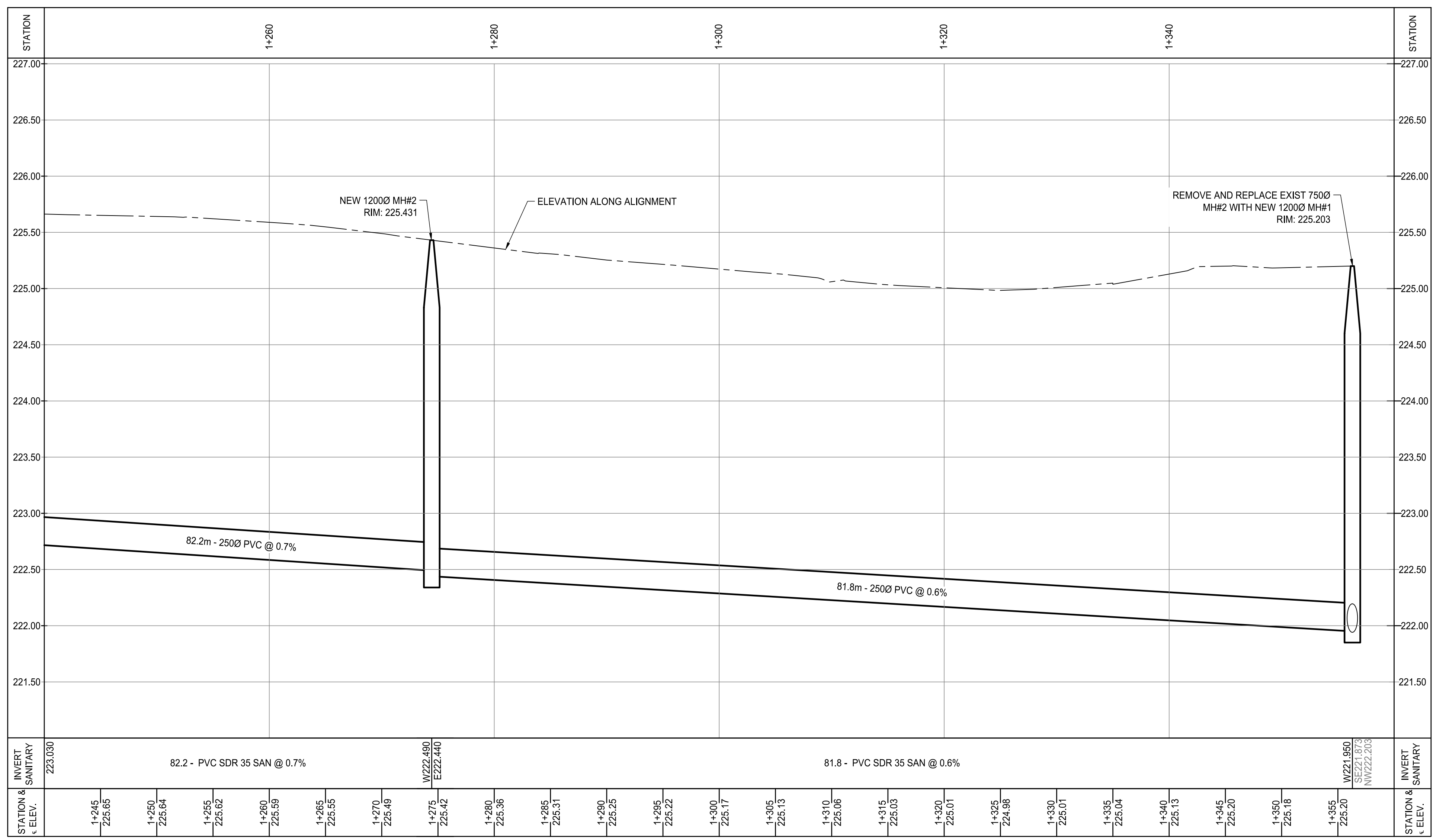
PROFILE STA 1+240 TO 1+360 SCALE: H:1:250 V:1:25
