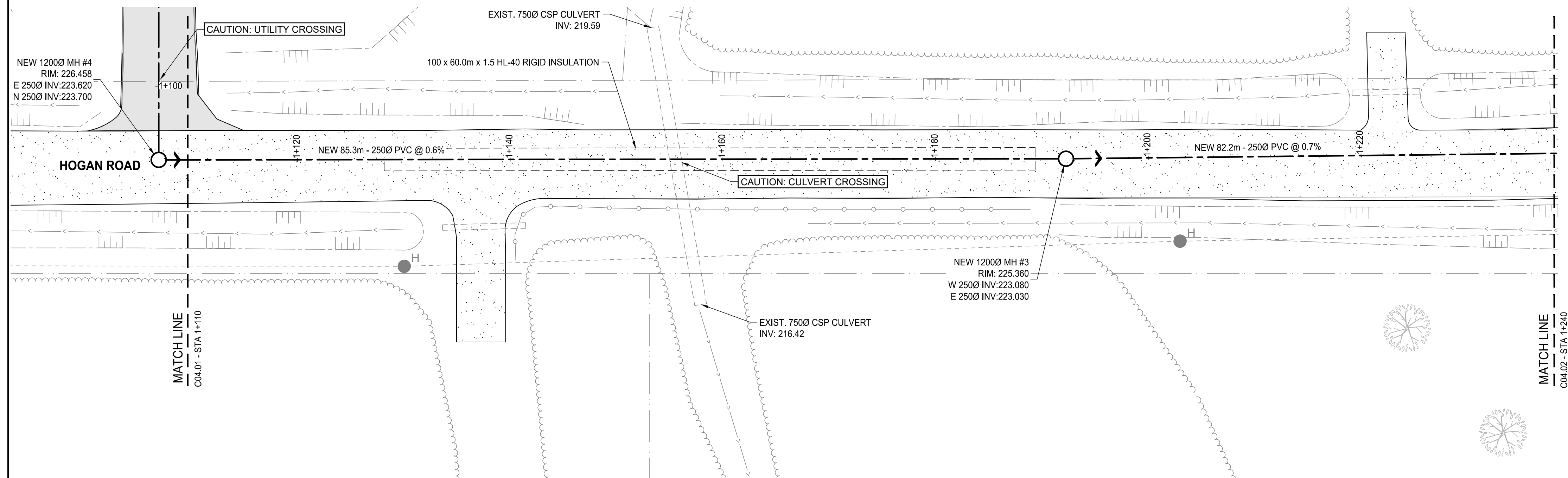
PLAN VIEW STA 1+110 TO 1+240 SCALE: 1:250
